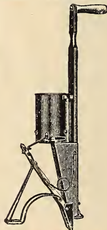
American Hand Corn Planter
